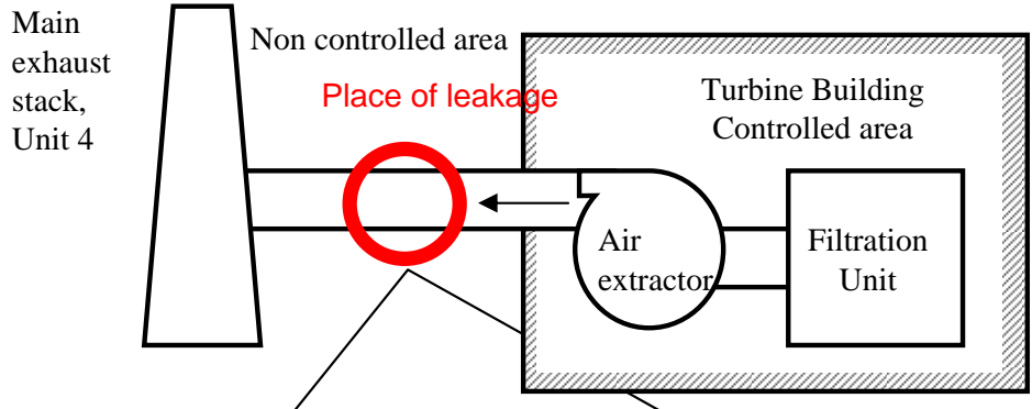
Air leakage at the welding with supporting legs, main exhaust duct, Unit 4 (Confirmed on June 7, 2011)
