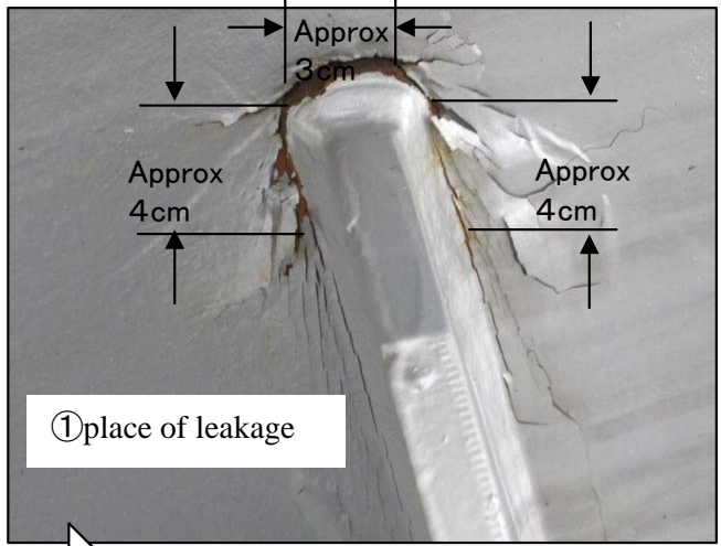
Air leakage at the welding with supporting legs, main exhaust duct, Unit 4 (Confirmed on June 7, 2011)
