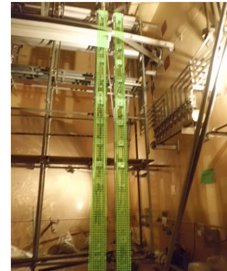
Steel support pillars (highlighted in color are pillars) *installed two pillars(among 32)
