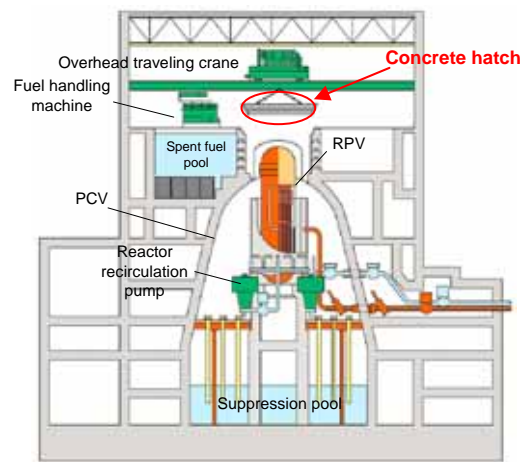
Reactor Building (Cross-section) (Concrete hatch removal)
