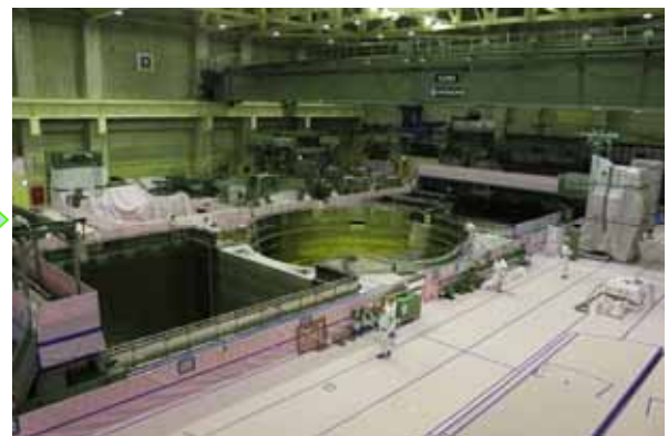
After the concrete hatch removal (Photo taken on September 10, 2012)
